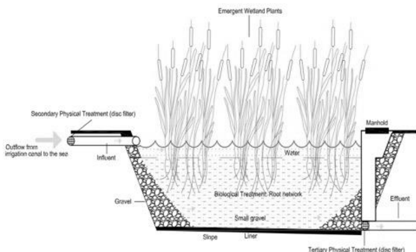
Figure 5 Constructed wetland in surface system
