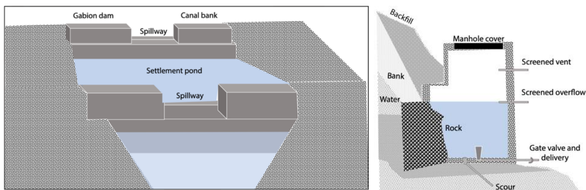
Figure 2 Check dam to control and store floodwater, combined with appended infiltration tank 85
